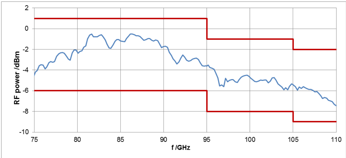
Test port output power versus frequency of the R&S®ZVA-Z110E.
